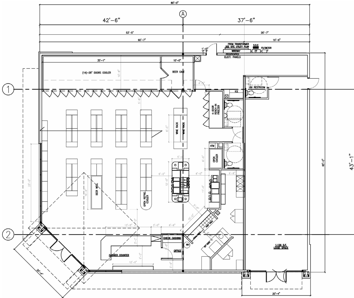
PRELIMINARY FLOOR PLAN 4450 E. OLD SETTLERS BLVD. ROUND ROCK, TEXAS
